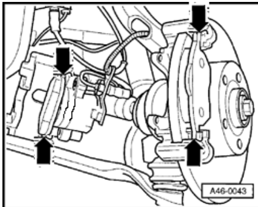
Figure 3. Contact points to be lubricated.
